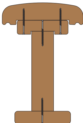
Big Rail Diagram
