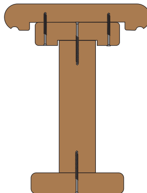
Flat Rail Diagram
